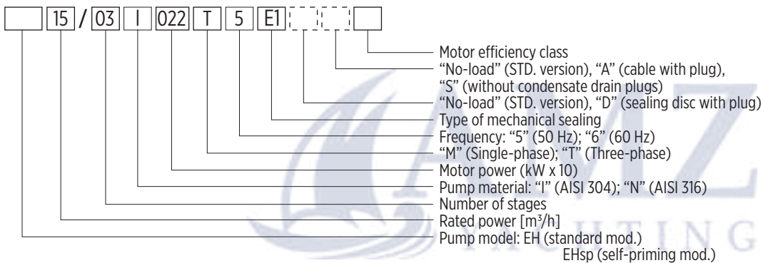
Fig. 2: Electric pump rating plate
